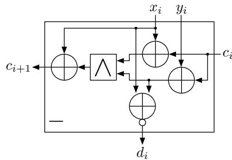
Fig. 4. Improved 1-bit Subtractor (−)
